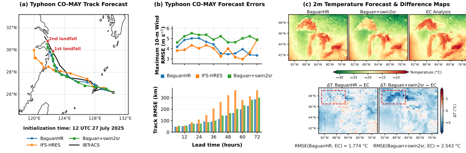
Fig. 8: (a) Typhoon CO-MAY tracking forecast, which is initialized at 12 UTC, 27 July 2025. (b) Forecast errors of track and intensity. (c) Case study of 2m temperature forecast over the U.S. Great Lakes region, initialized at 00 UTC, 20 January 2025.
